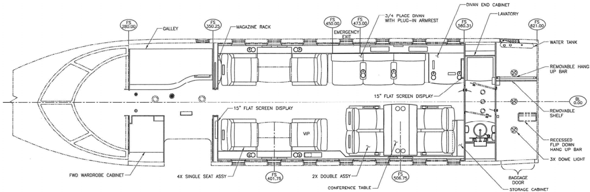
FLOOR PLAN EXTENDED CABIN OPPOSING LAVATORY
